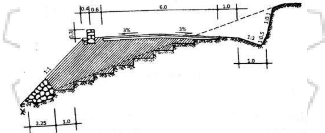
Typical Cross Sections of Cut and fill
