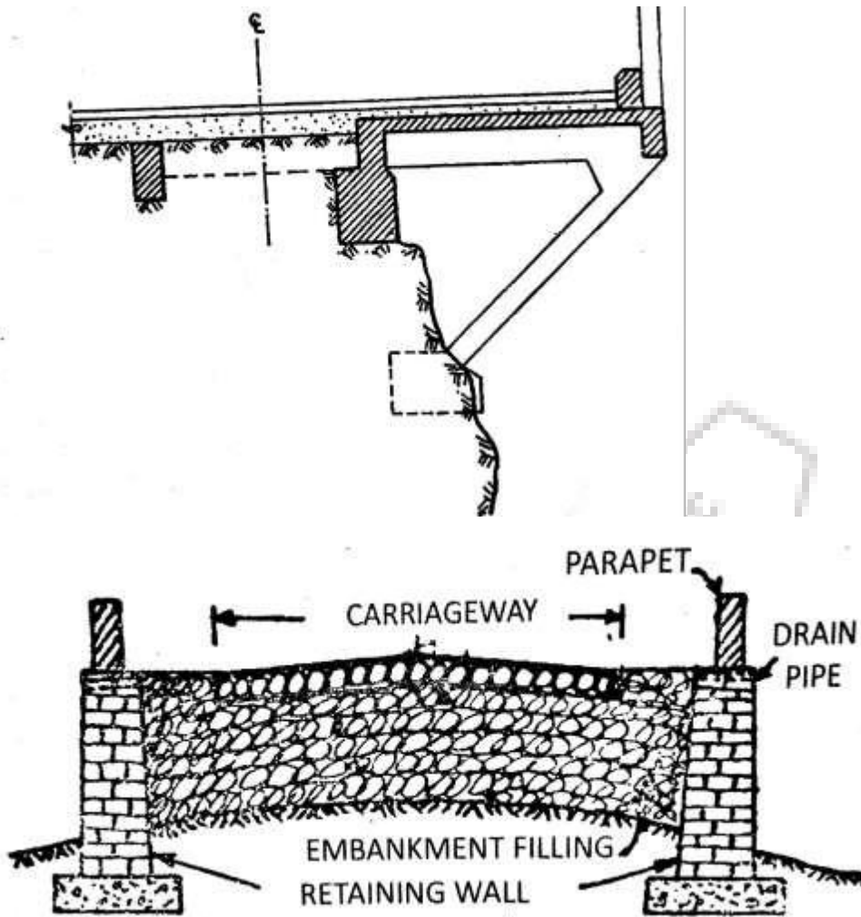
Fig: Fully In Embankment
