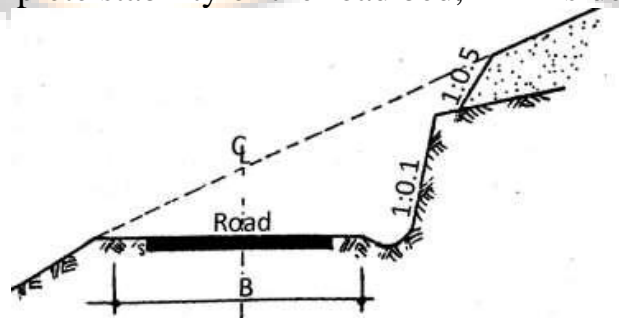
Typical Cross Sections of Bench type
