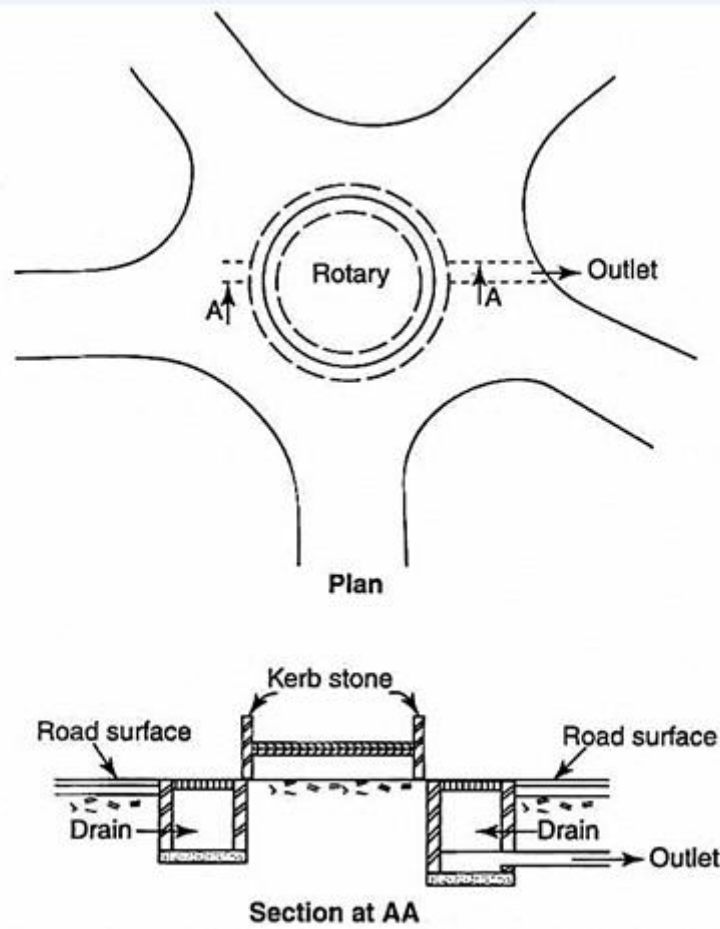
Fig. Typical drainage arrangement at a Rotary
